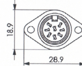
THROUGH HOLE DIMENSIONS
