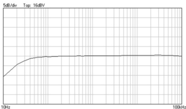
Frequenzgang @ 8 Ohm
