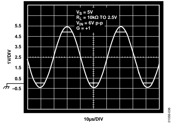
Figure 36. Output Voltage
