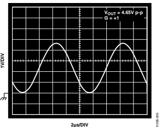
Figure 5. Output V_{OUT}
